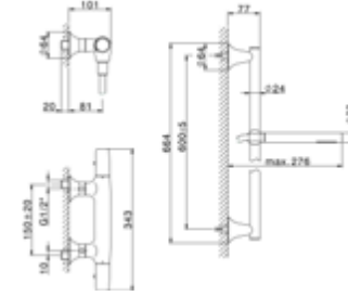
VI S01010 Completo Termostatico Doccia Thermo Shower Set Ensemble Thermo Douche
