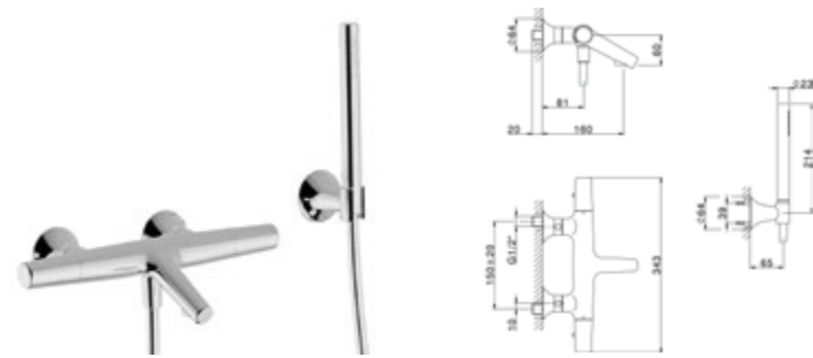
VI D21010 Completo Termostatico Vasca Thermo Bath/S. Set Ensemble Thermo Bain/D.
