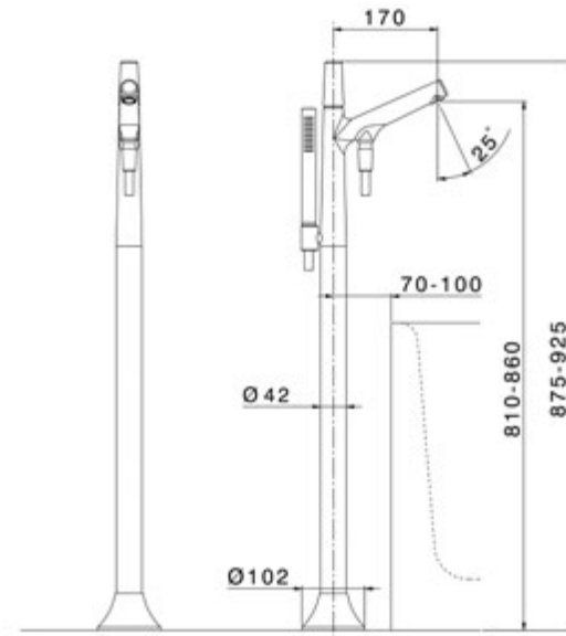
VI 014204 Parte Esterna Monocomando Vasca Free-Standing Free-Standing Bath/S. Mixer Exposed Part Partie Apparente Mitigeur Bain/D. Free-Standing Vedi / See / Voir ZA 004510
